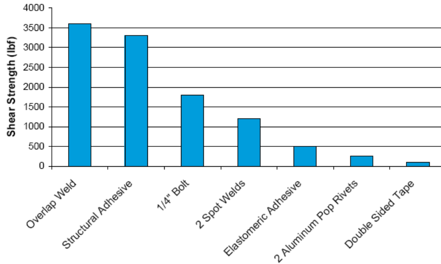
FIGURE 1: Shear Strength for Various Assembly Methods
