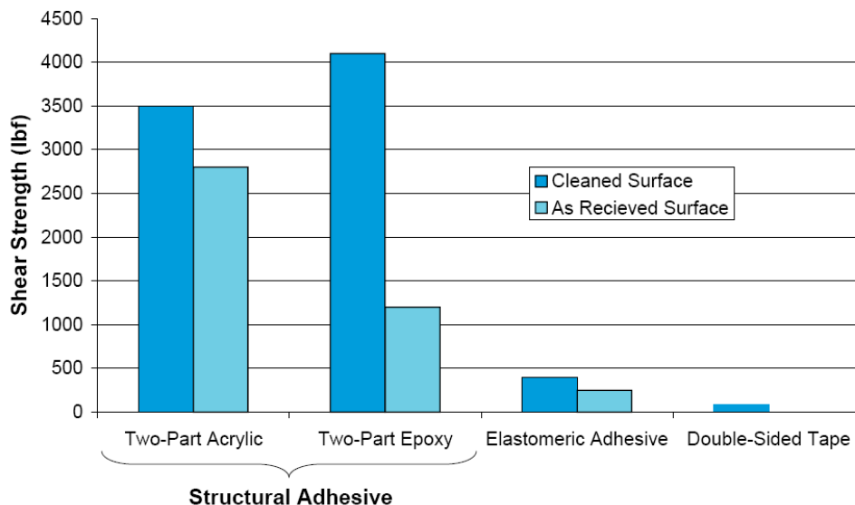
FIGURE 4: Shear Strength on Cleaned vs. As Received Steel
