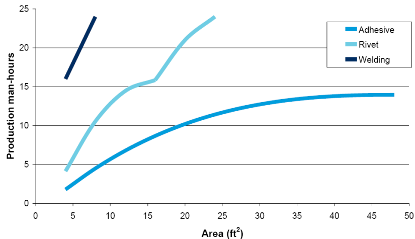
FIGURE 2: Man-hours vs. Assembled Area for Various Fastening Methods
