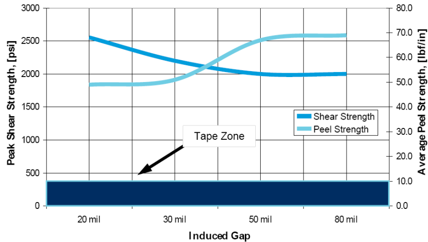
Figure 6: Effect of Varying Induced Gap on Shear and Peel Strength of Structural Adhesives
