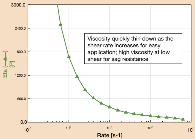
Shear-Thinning of PG-V
