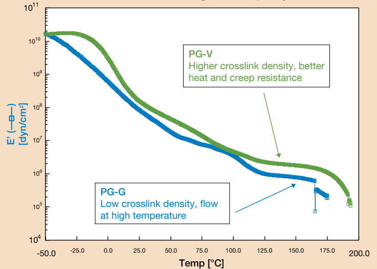
Cured Rheological Property
