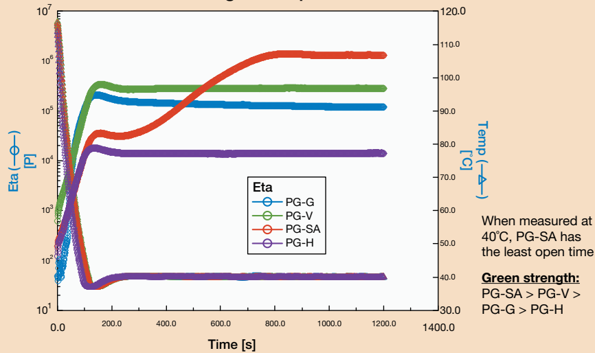
Green Strength Comparison
