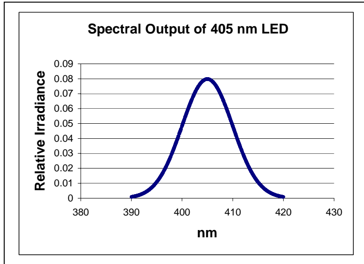
Figure 2 -Spectral Output Distribution for a 405 nm Based LED Light Source
